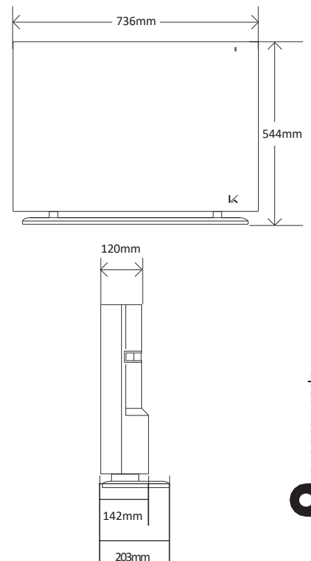
● Dimension Drawing (mm)
